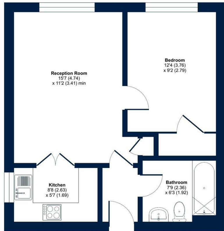
FIRST FLOOR
